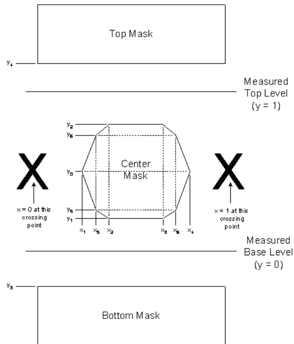
Figure 32. Mask Definition
