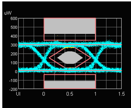
Mask margin for 91 failing points: +61 %
