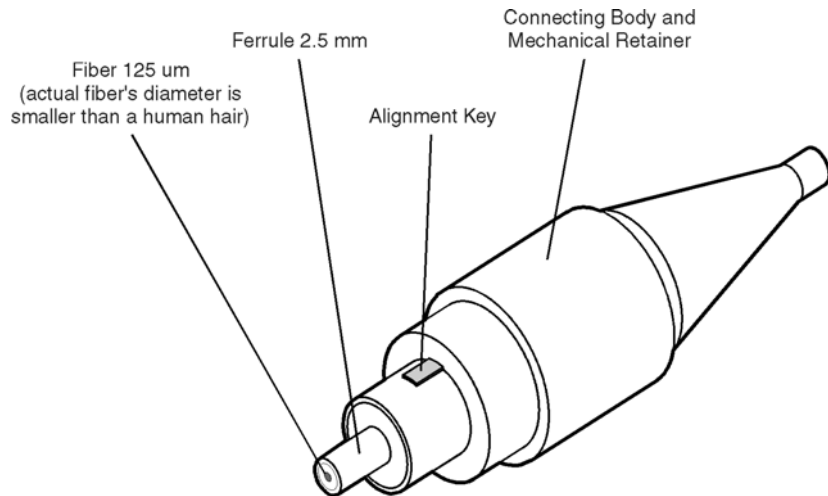
Figure 3. Basic components of a connector.
