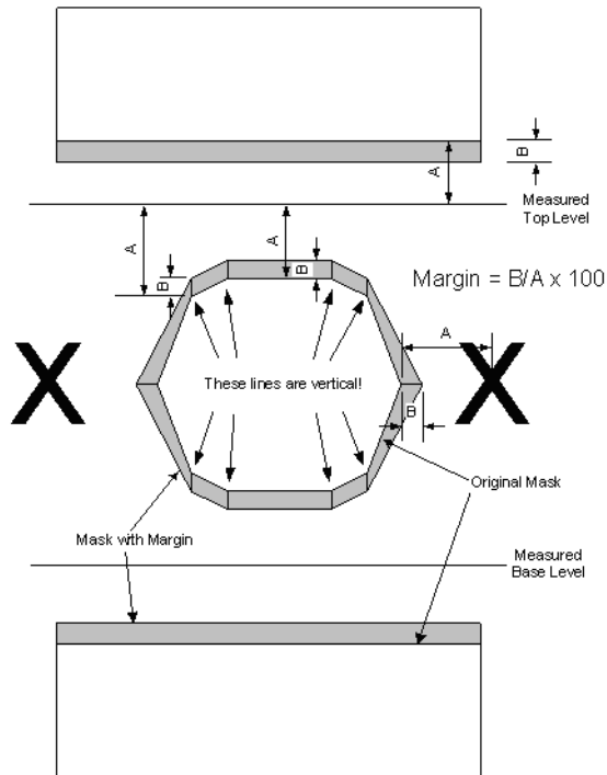
Figure 35. Agilent Mask - Positive Margin
