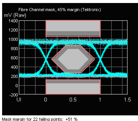
Figure 18. Find Max Mask Margin
