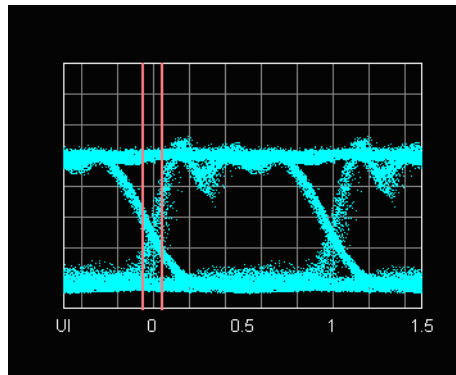
Jitter 41.5 ps Peak to Peak, 7.8 ps RMS
