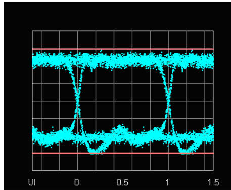
Peak to peak 734.4 mV
