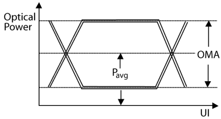
Figure 14. Optical Power
