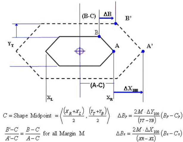
Figure 38. Tektronix Margin Rules for 6- and 10-Point Masks
